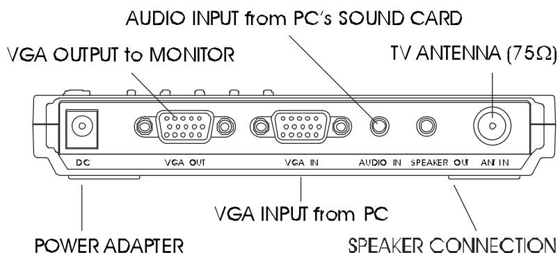
AVerMedia AVerTV Box5 Live Back Panel
