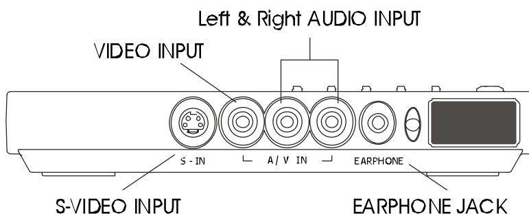
AVerMedia AVerTV Box5 Live Front Panel
